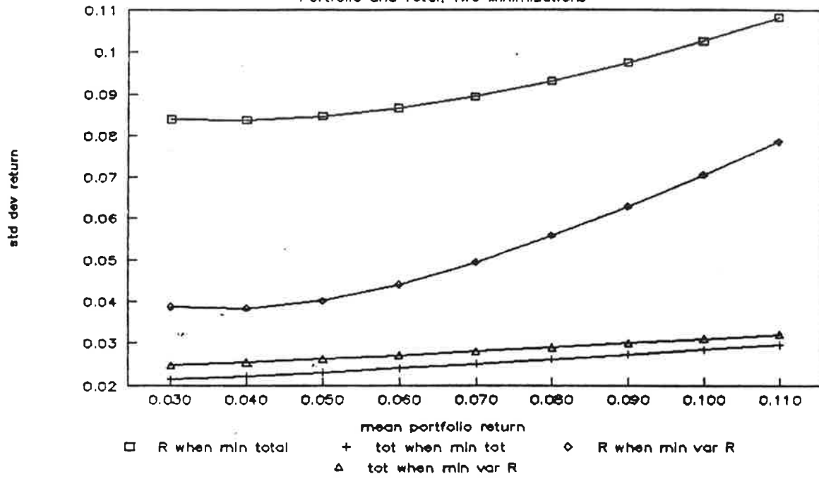
Fig. A-3 Comparing Risk-Return Loci Portfolio and Total, Two Minimizations
