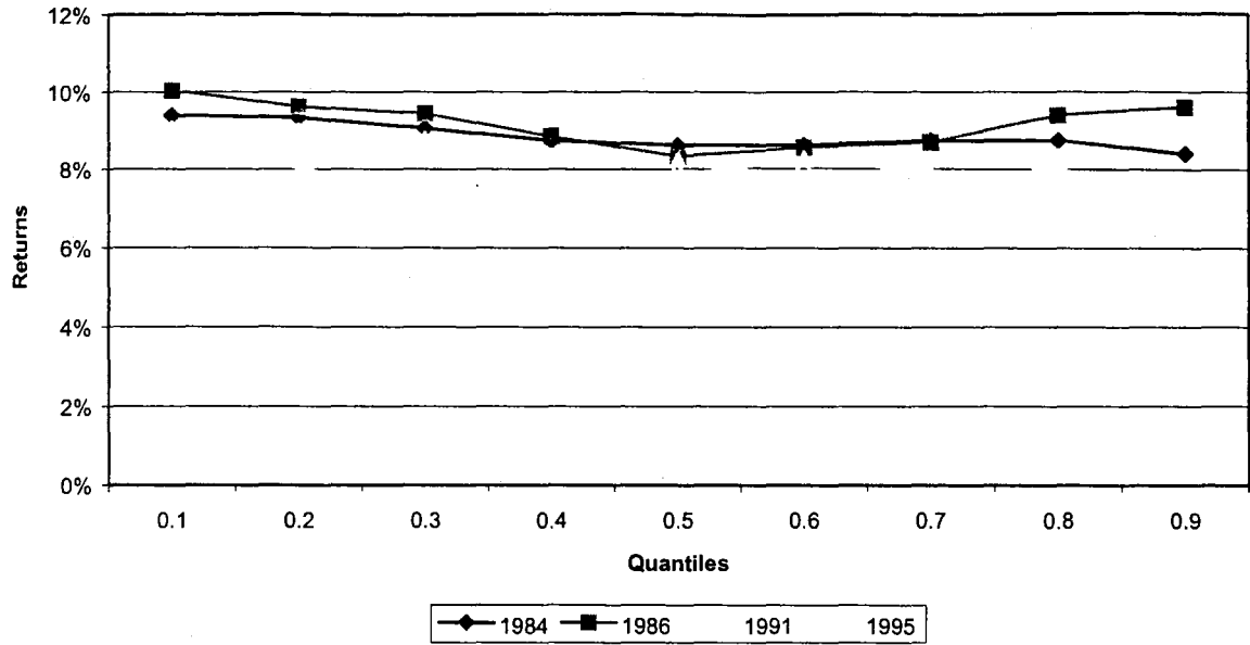
Graph 5.5 - Returns to Education in Germany, 1984-1995 Quantile regressions
